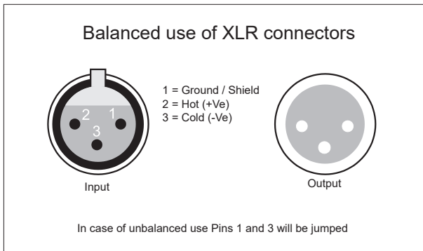
Fig. 5.1 XLR connector
